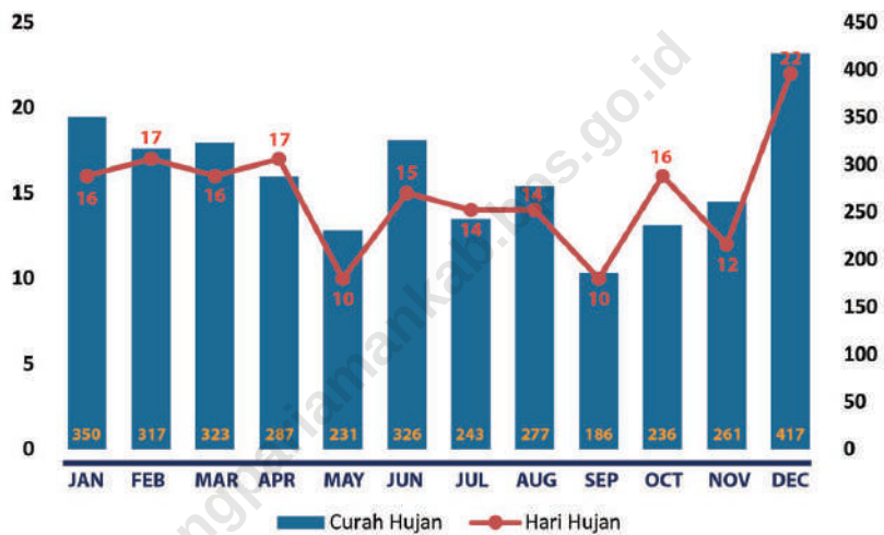
Gambar 1.3 Rata-rata Curah Hujan per Bulan di Kabupaten Padang Pariaman, 2019 Figures Average of Rainfall by Month at Padang Pariaman Regency, 2019(mm)
